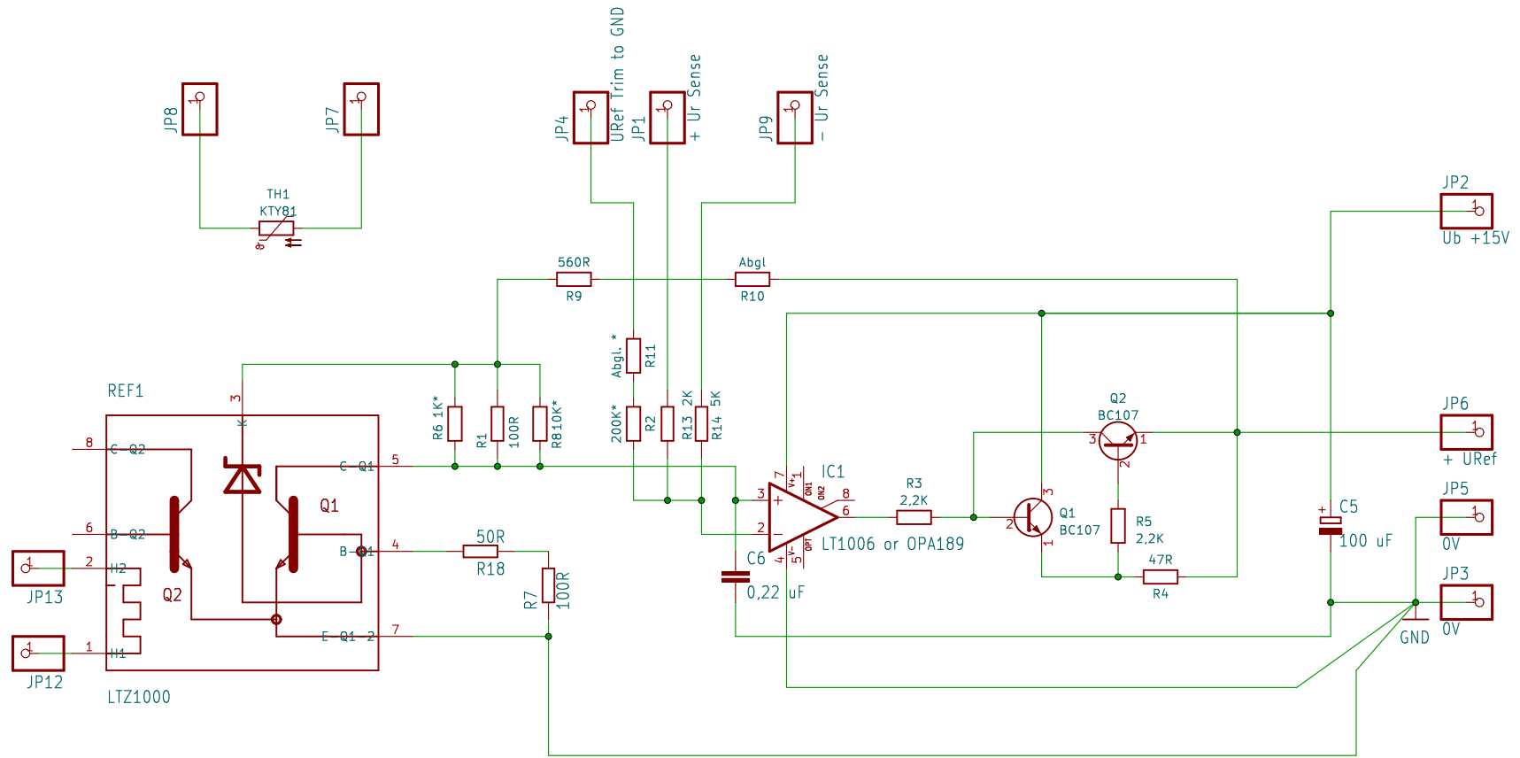
LTZ1000 10V DC Reference-Standard (without heater) FM 01/2024
